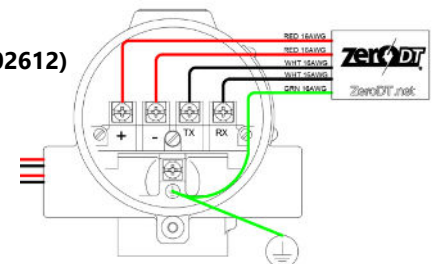
Dual Loop or 4-Wire Devices ZeroDT 24-2 & ZeroDT 12-2 2 Red Wire ( Voltage + or - ) 2 White Wire ( Voltage + or - ) 1 Green Wire (GND)
